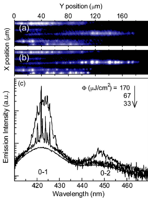
FIG. 2. (Color online) Time integrated optical emission micrographs of nanofibers excited by ultrafast pulses, for a pump fluence of 33 (a) and 170 \mu\text{J}/\text{cm}^2 per pulse (b). Panel (c) Time integrated emission spectra of the nanofiber placed at the center of the X position range in panels (a) and (b), for different values of the excitation fluence. The spectra are spatially integrated over the nanofiber region (from Y \approx 10 \mu\text{m} to Y \approx 185 \mu\text{m} ).
